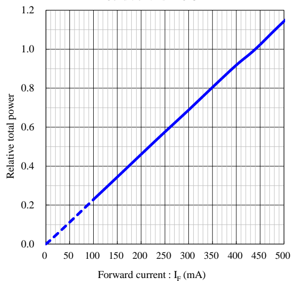
Forward current vs. Relative total power
