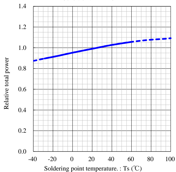
Soldering point temp. vs. Relative total power
