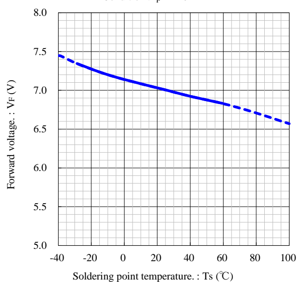
Soldering point temp. vs. Forward voltage
